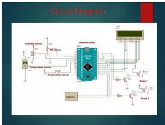
Fig1. Water quality monitoring system
